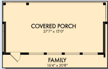
OPTIONAL EXTENDED COVERED PORCH
