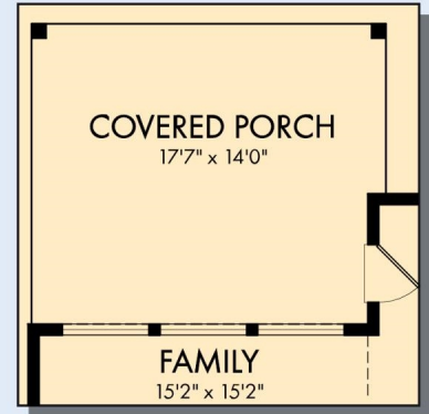
OPTIONAL EXTENDED COVERED PORCH
