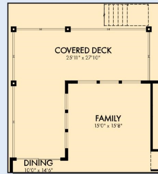
OPTIONAL EXTENDED COVERED DECK WITH DAYLIGHT/WALKOUT BASEMENT
