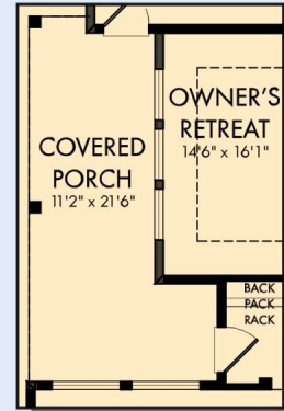
OPTIONAL EXTENDED COVERED PORCH
