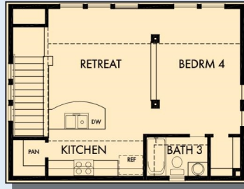
OPTIONAL GARAGE RETREAT WITH BEDROOM 4 AND BATH 3 ABOVE ATTACHED 2 CAR GARAGE
