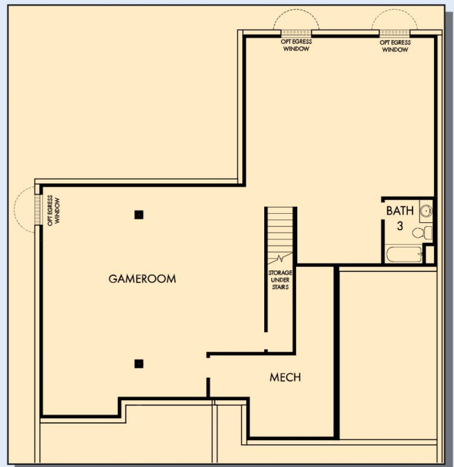
OPTIONAL GAME ROOM WITH BATH 3 AT BASEMENT
