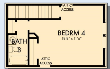
SECOND FLOOR WITH OPTIONAL BONUS WITH BEDROOM 4 AND BATH 3
