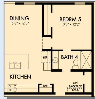
OPTIONAL BEDROOM 5 WITH BATH 4 AT SITTING
