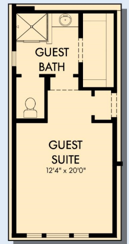
OPTIONAL GUEST SUITE AT BEDROOM 2 AND STUDY
