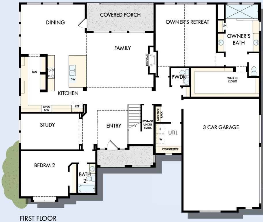
FIRST FLOOR
