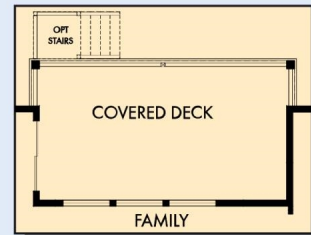
OPTIONAL EXTENDED COVERED DECK WITH DAYLIGHT/WALKOUT BASEMENT
