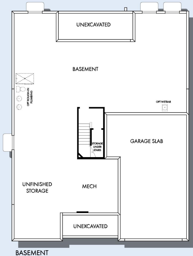
BASEMENT
