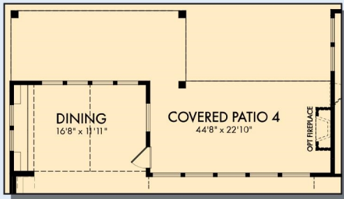
OPTIONAL COVERED PATIO 4
