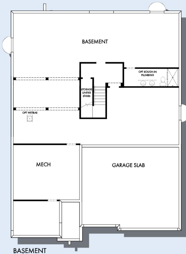
BASEMENT
