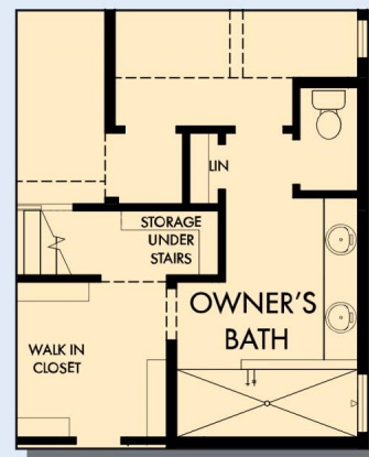
OPTIONAL SUPER SHOWER AT OWNER'S BATH
