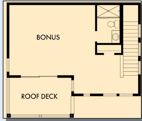
OPTIONAL THIRD FLOOR BONUS WITH FRONT ROOF DECK AND BATH 3
