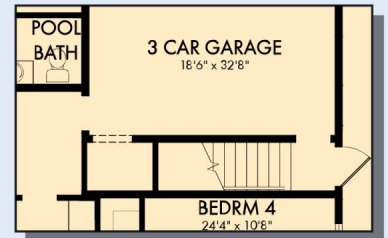
FIRST FLOOR WITH OPTIONAL SECOND FLOOR RETREAT ABOVE 3 CAR GARAGE
