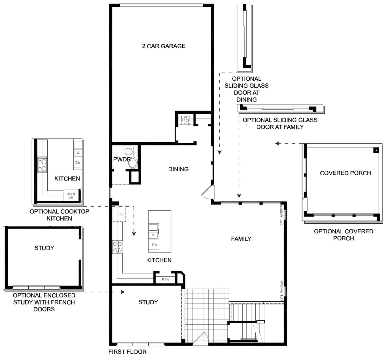
FIRST FLOOR
