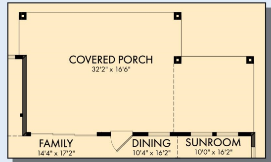
OPTIONAL EXTENDED COVERED PORCH WITH SLIDING GLASS DOOR AT FAMILY
