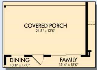
OPTIONAL EXTENDED COVERED PORCH WITH SLIDING GLASS DOOR AT FAMILY
