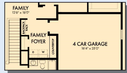
FIRST FLOOR WITH OPTIONAL BASEMENT
