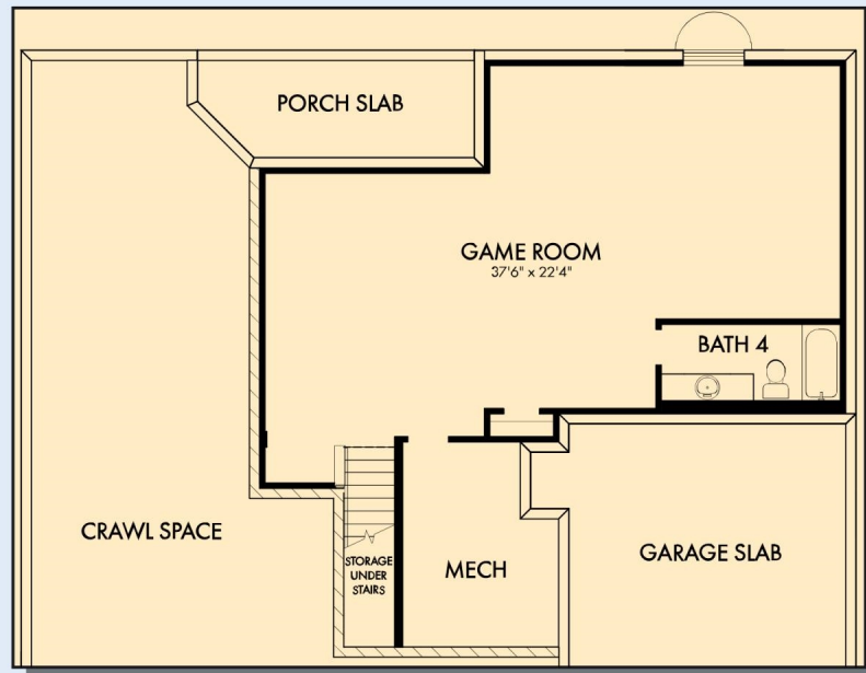
OPTIONAL GAME ROOM WITH BATH 4 AT BASEMENT
