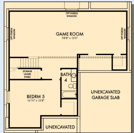
OPTIONAL GAMEROOM WITH BEDROOM 5 AND BATH 4 AT BASEMENT
