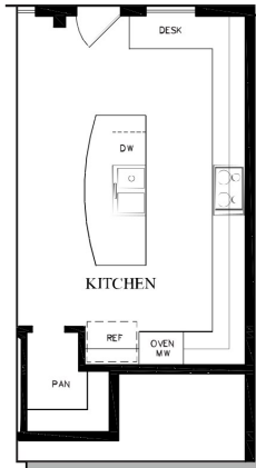
OPTIONAL COOKTOP KITCHEN
