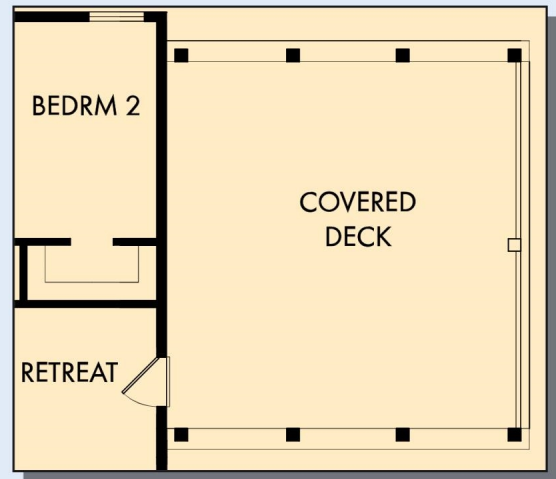
OPTIONAL COVERED DECK AT RETREAT
