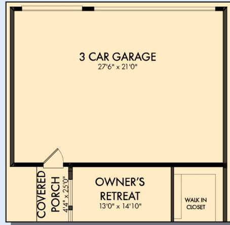
OPTIONAL 3 CAR GARAGE
