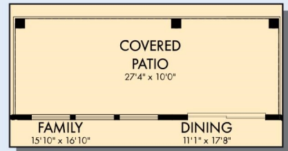
OPTIONAL EXTENDED COVERED PATIO AT FAMILY AND DINING
