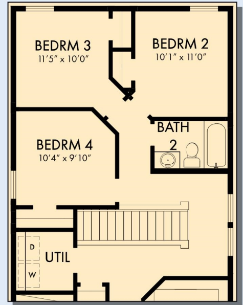
OPTIONAL BEDROOM 4 AT RETREAT
