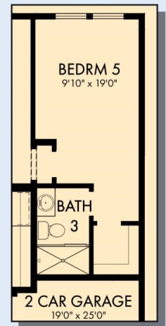
OPTIONAL BEDROOM 5 WITH BATH 3 AT KEEPING ROOM
