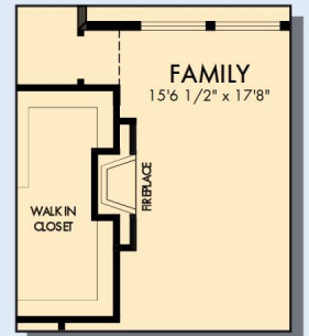
OPTIONAL WALL FIREPLACE AT FAMILY
