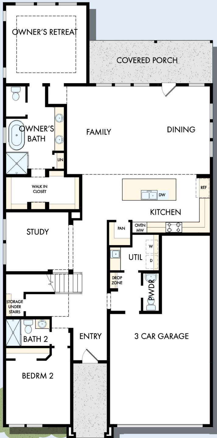
FIRST FLOOR
