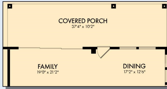
OPTIONAL EXTENDED COVERED PORCH WITH SLIDING GLASS DOOR AT FAMILY
