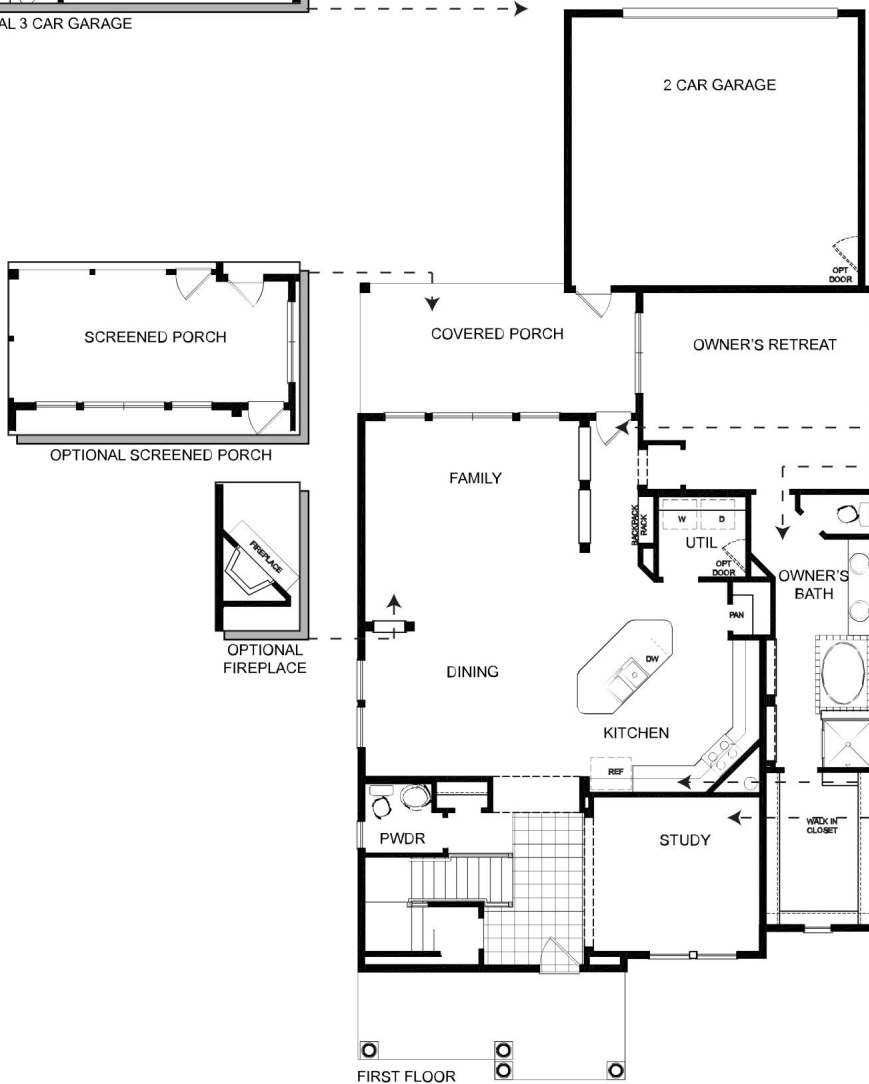
FIRST FLOOR
