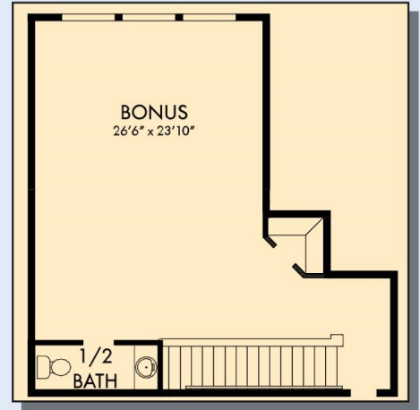
OPTIONAL SECOND FLOOR BONUS WITH HALF BATH
