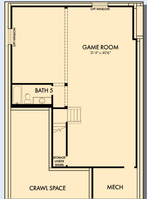
OPTIONAL GAME ROOM WITH BATH 5 AT BASEMENT
