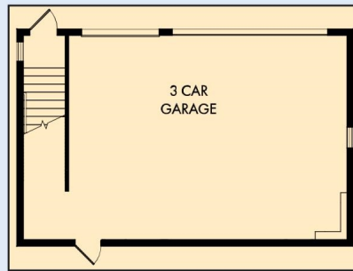
FIRST FLOOR WITH OPTIONAL GARAGE RETREAT ABOVE 3 CAR DETACHED GARAGE
