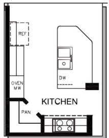
OPTIONAL COOKTOP KITCHEN WITH STACKED OVEN/MICROWAVE
