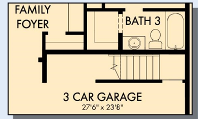
FIRST FLOOR WITH OPTIONAL WALK UP STORAGE
