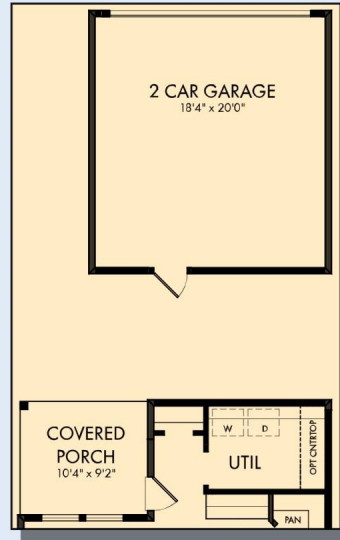
OPTIONAL DETACHED 2 CAR GARAGE
