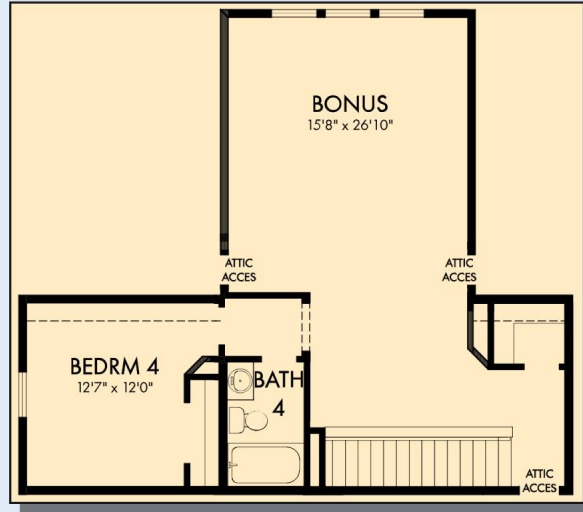
OPTIONAL SECOND FLOOR BONUS WITH BEDROOM 4 AND BATH 4
