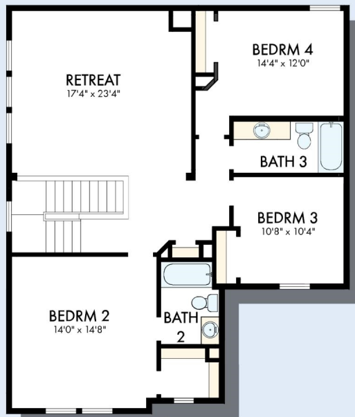
SECOND FLOOR
