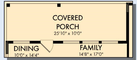
OPTIONAL COVERED PORCH
