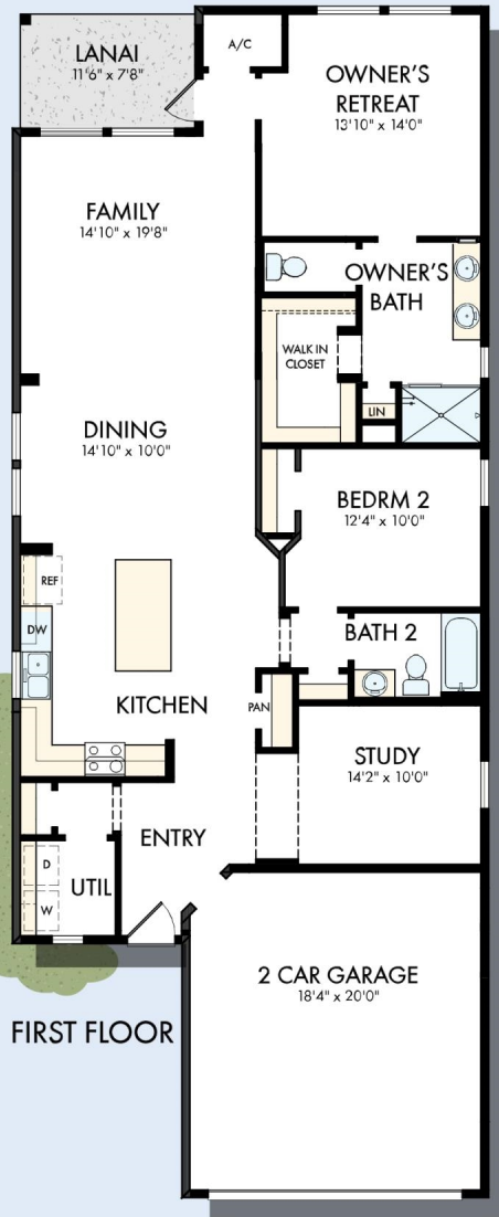
OPTIONAL EXTENDED LANAI WITH SLIDING GLASS DOOR
