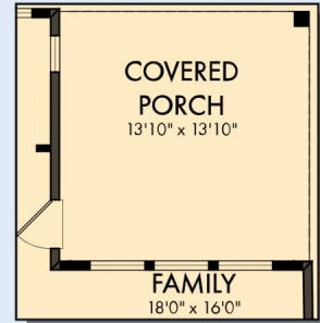
OPTIONAL EXTENDED COVERED PORCH
