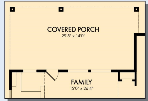
OPTIONAL EXTENDED COVERED PORCH AT FAMILY
