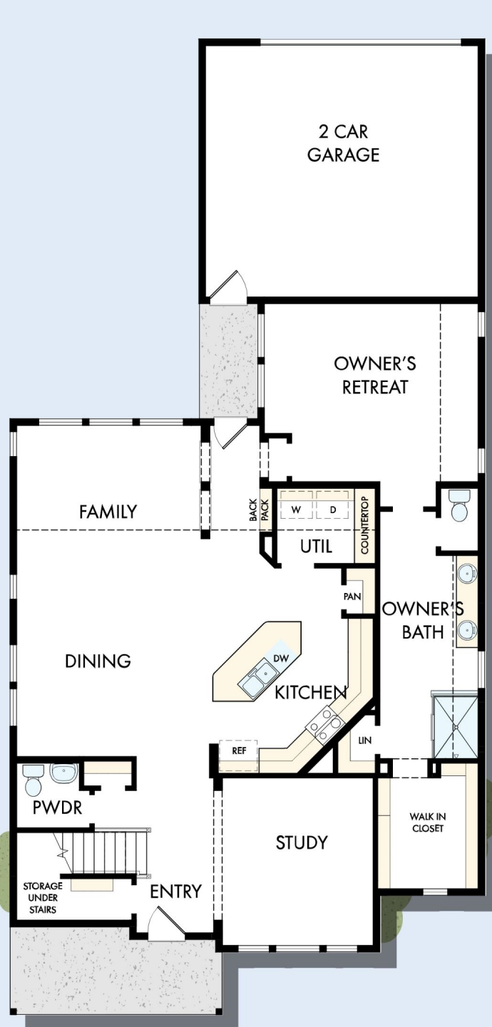
FIRST FLOOR
