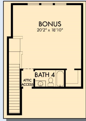
OPTIONAL SECOND FLOOR BONUS WITH BATH 4
