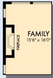
OPTIMAL WALL FIREPLACE AT FAMILY
