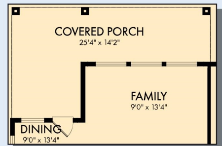
OPTIONAL EXTENDED COVERED PORCH AT FAMILY
