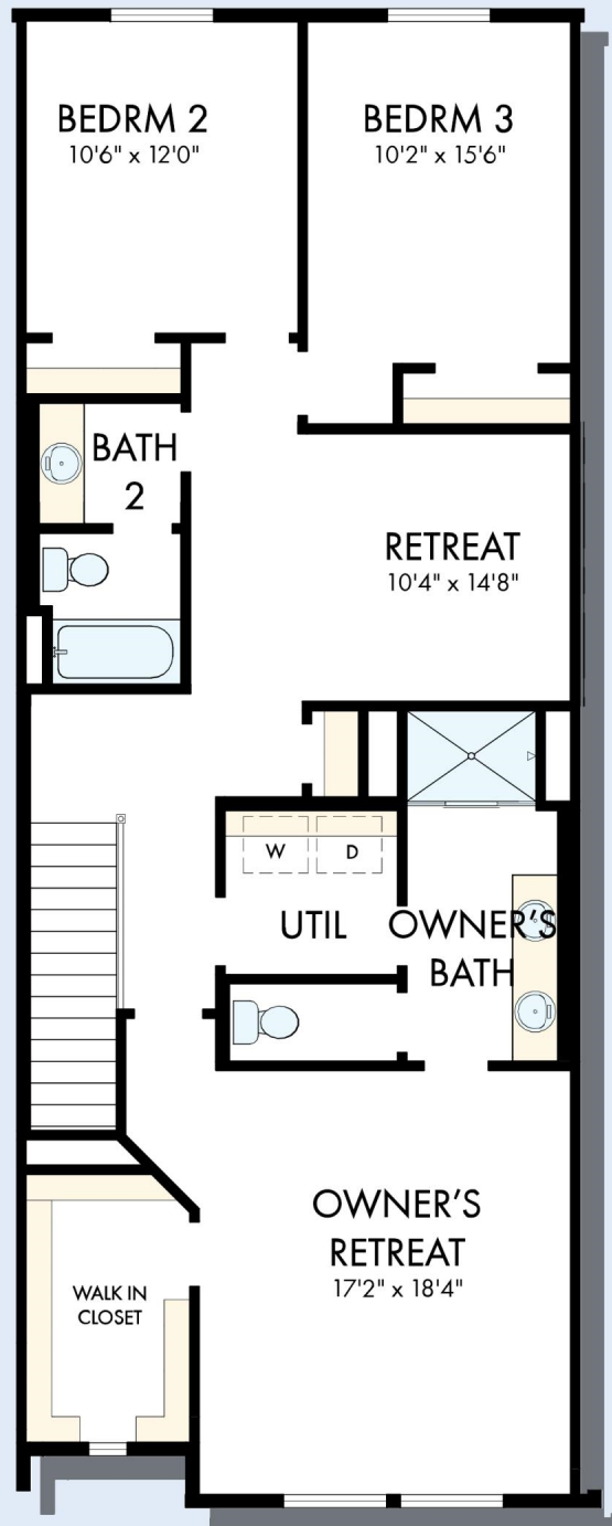
SECOND FLOOR
