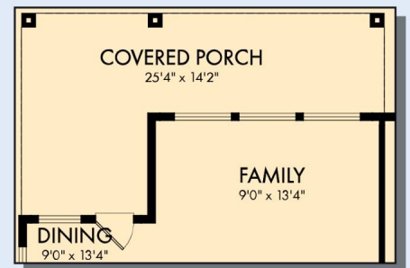
OPTIONAL EXTENDED COVERED PORCH AT FAMILY
