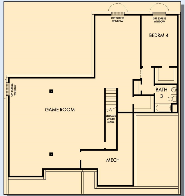
OPTIONAL GAME ROOM WITH BEDRM 4 AND BATH 3 AT BASEMENT
